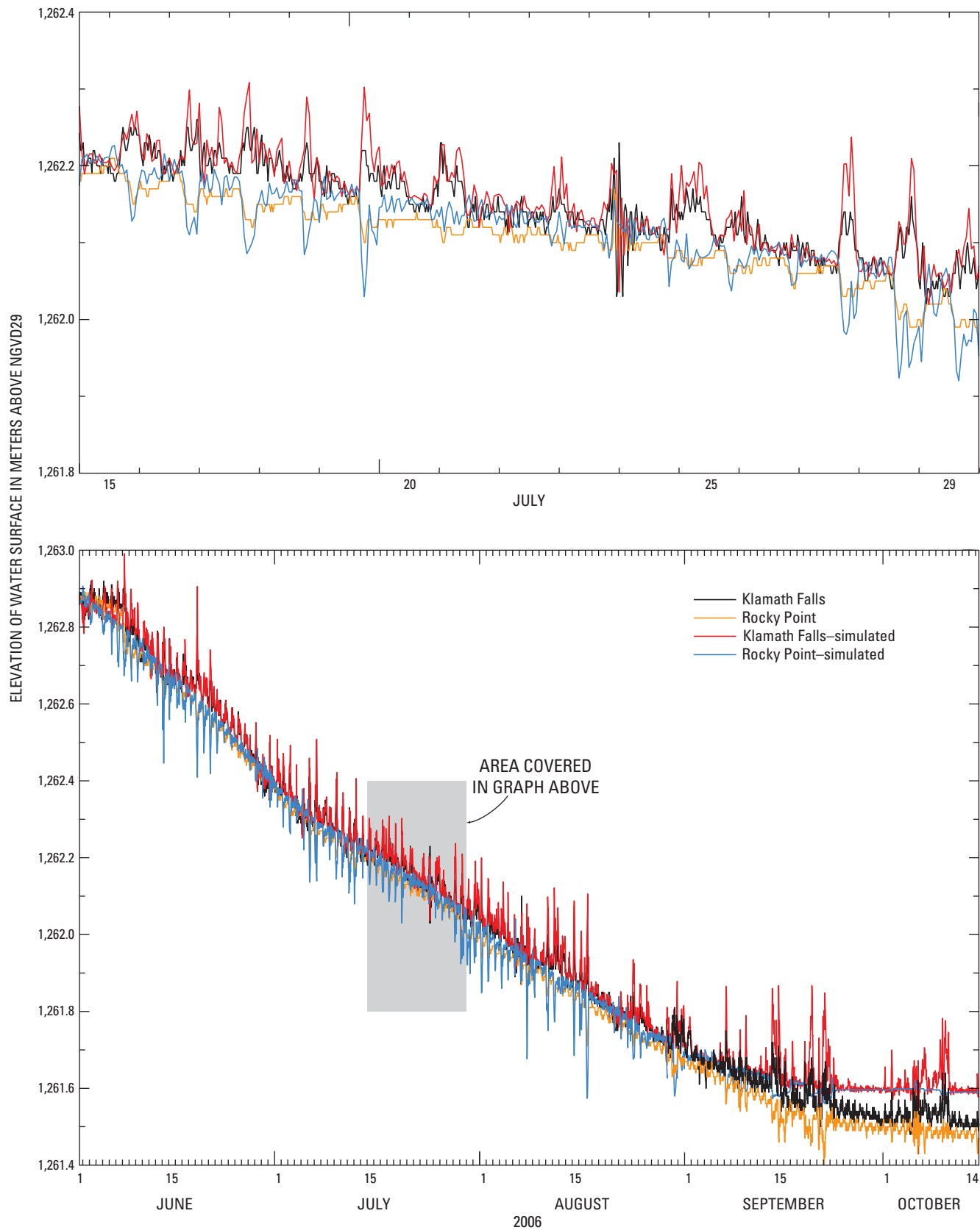
Figure 14. Hourly values of lake elevation at Upper Klamath Lake, Oregon, measured at two gages, 2006.
